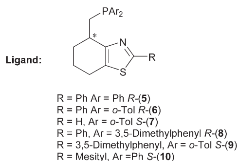
Figure 1. Phosphine-thiazole ligands used in the asymmetric intermolecular Heck reaction.
