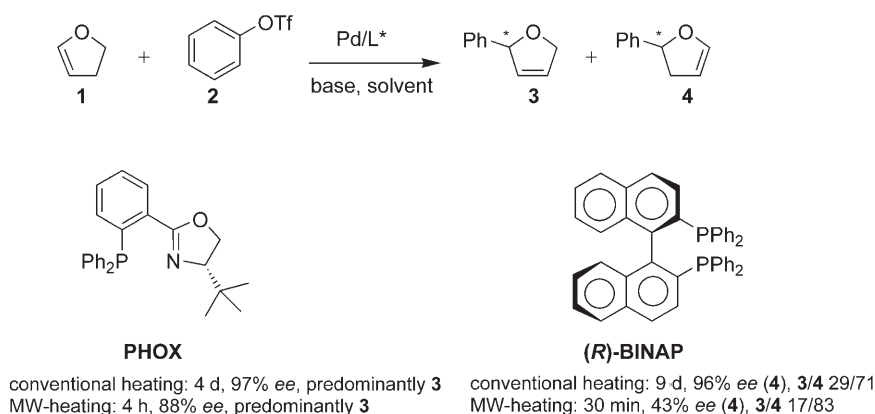
Scheme 1. The asymmetric intermolecular Heck reaction with 2,3-dihydrofuran and phenyl triflate.
