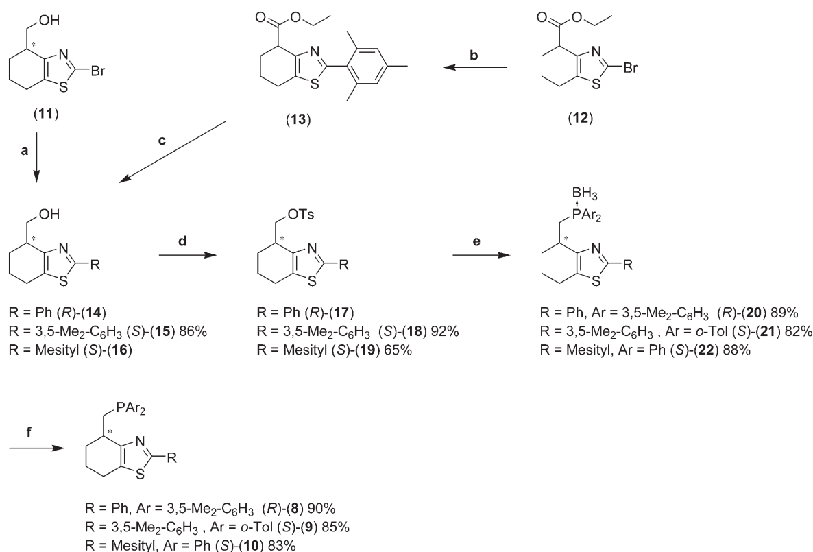
Scheme 2. Reagents and conditions: a) ArB(OH) 2 , DPPF-PdCl 2 (5 mol %), K 2 CO 3 (aqueous), toluene, 80 °C; b) SPHOS (8 mol %), Pd 2 (dba) 3 (4 mol %), mesitylB(OH) 2 , K 3 PO 4 , toluene, reflux, overnight, 95 %; c) LiAlH 4 , THF, r.t., overnight, then preparative HPLC, Chiracel OD; d) TsCl, pyridine, 0 °C to r.t. overnight; e) Ar 2 P(BH 3 )H, n -BuLi, THF, DMF, −78 °C to r.t. overnight; f) Et 2 NH, r.t., overnight.
